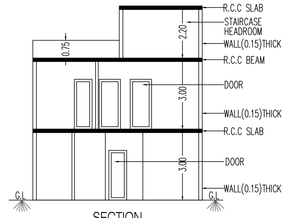
SECTION
